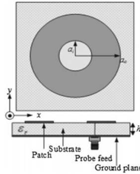
Figure 19. Circular ring compact microstrip antenna structure
