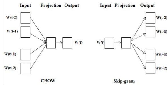
Figure 3. Structure of Skip – Gram and CBOW (Suleiman & Awajan, 2019)
