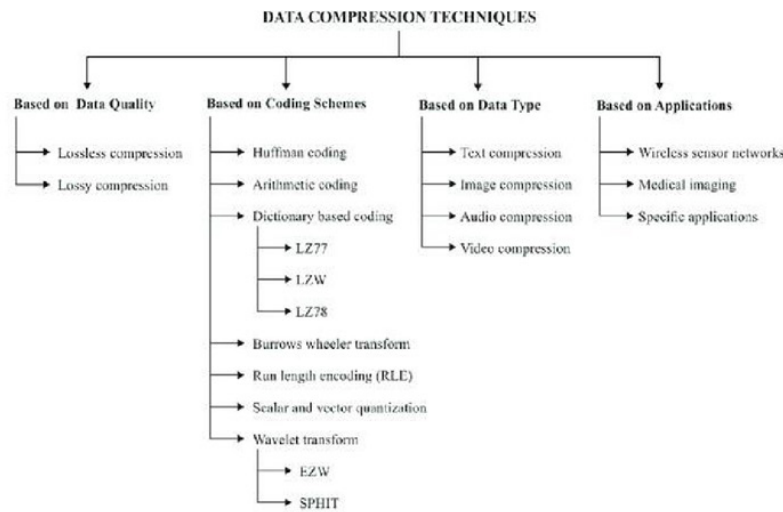
Figure 2 Data Compression Techniques (Jayasankar, 2021).
